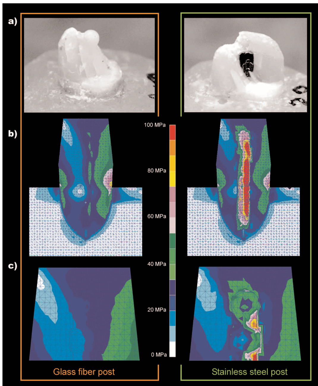
Figure 5: Results: a) detail of the experimental fractures on the restored teeth; b) estimated Von Mises stress distribution patterns; c) detail of the estimated Von Mises stress distribution patterns on the composite core.
