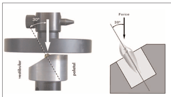
Figure 1: Experimental fracture strength test performed on teeth.
