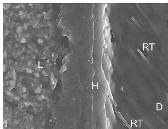
Figure 7. Scanning electron micrographs of the interfacial layers between dentin and the resin based luting agent in Group I C. D, dentin; L, luting agent; H, hybrid zone; RT, resin tag (original magnification 3000x).
