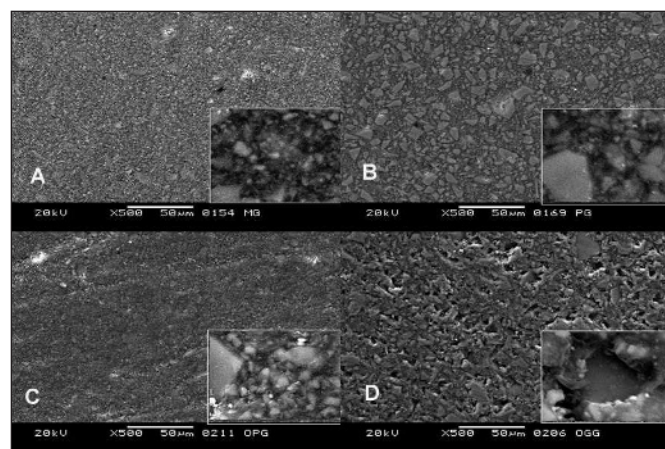
Figure 4. Grandio surfaces polished with different one-step polishing systems (500x magnification; 5000x in the box). Figure 4A. Control surface (Mylar); B. Polished with PoGo; C. Polished with OptraPol; D. Polished with One Gloss.
