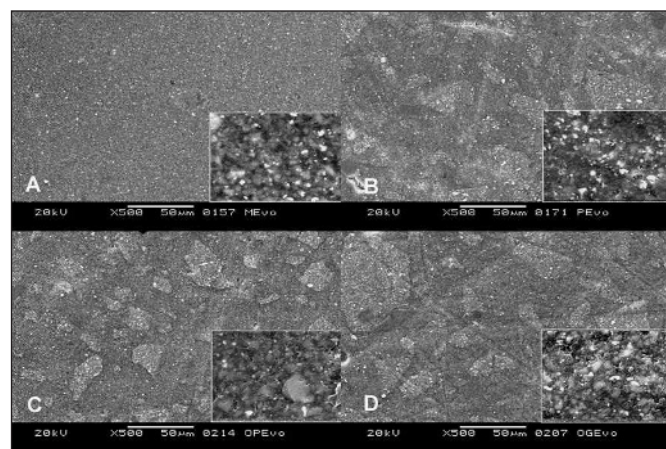
Figure 2. Tetric EvoCeram surfaces polished with different one-step polishing systems (500x magnification; 5000x in the box). Figure 2A. Control surface (Mylar); B. Polished with PoGo; C. Polished with OptraPol; D. Polished with One Gloss.
