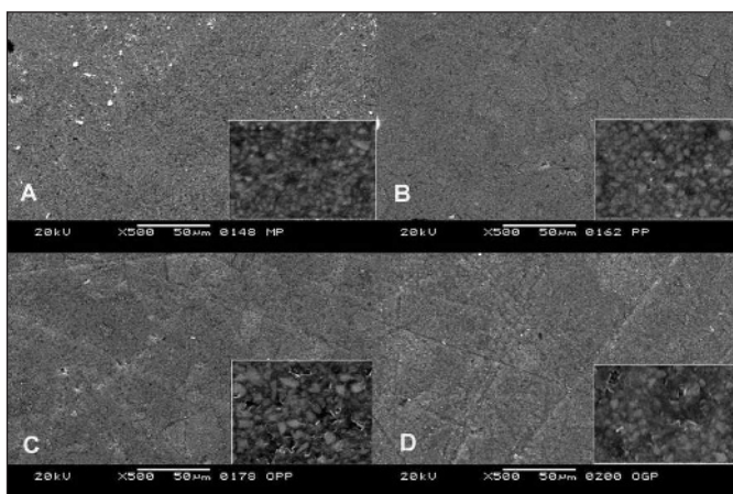
Figure 3. Premise surfaces polished with different one-step polishing systems (500x magnification; 5000x in the box). Figure 3A. Control surface (Mylar); B. Polished with PoGo; C. Polished with OptraPol; D. Polished with One Gloss.
