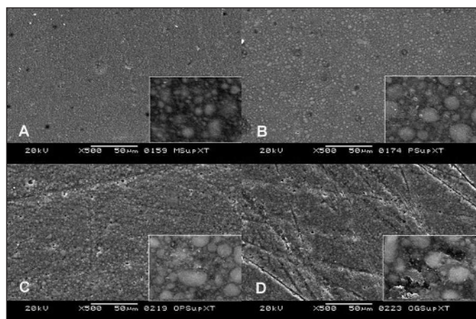
Figure 1. Filtek Supreme XT surfaces polished with different one-step polishing systems (500x magnification; 5000x in the box). Figure 1A. Control surface (Mylar); B. Polished with PoGo; C. Polished with OptraPol; D. Polished with One Gloss.
