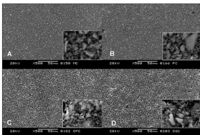
Figure 5. CeramX surfaces polished with different one-step polishing systems (500x magnification; 5000x in the box). Figure 5A. Control surface (Mylar); B. Polished with PoGo; C. Polished with OptraPol; D. Polished with One Gloss.
