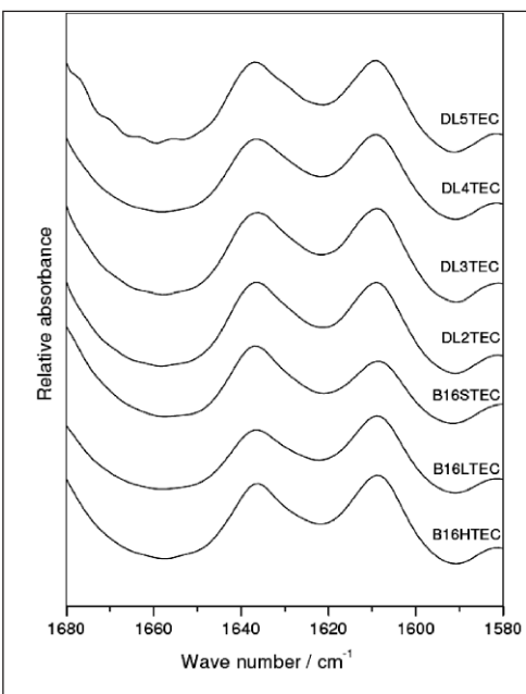
Figure 5: Polymerization spectra of TEC composite material polymerized with different curing modes.
