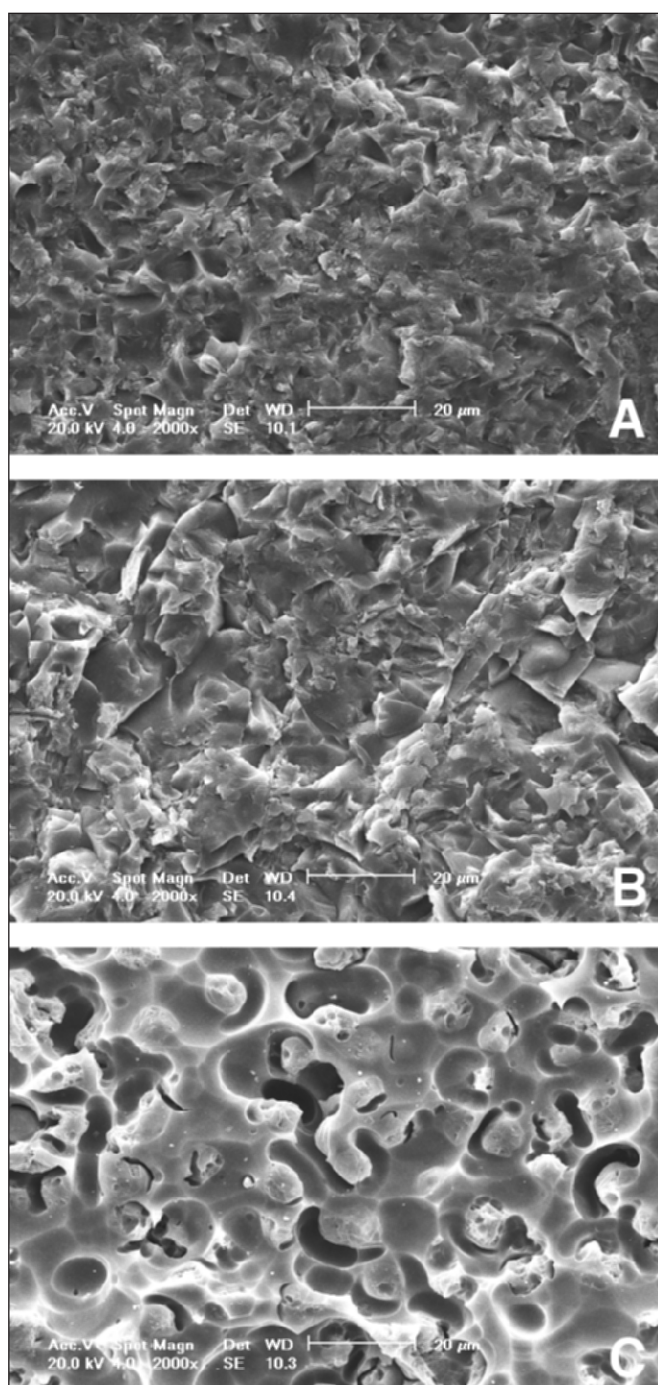
Figure 4. SEM of Cergogold (a) Control (original magnification 2000x), (b) Airborne particle abrasion with 50- \mu m aluminum oxide for 15 seconds (original magnification 2000x), (c) Etching with 9.5% of hydrofluoric acid for 60 seconds (original magnification 2000x).
