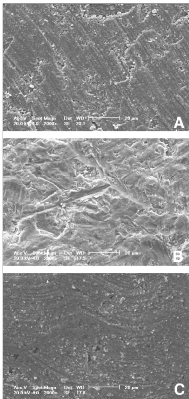
Figure 6. (a) SEM of Cercon (a) Control (original magnification 2000x) (b), Airborne particle abrasion with 50- \mu m aluminum oxide for 15 seconds (original magnification 2000x), (c) Etching with 9.5% of hydrofluoric acid for two minutes (original magnification 2000x).
