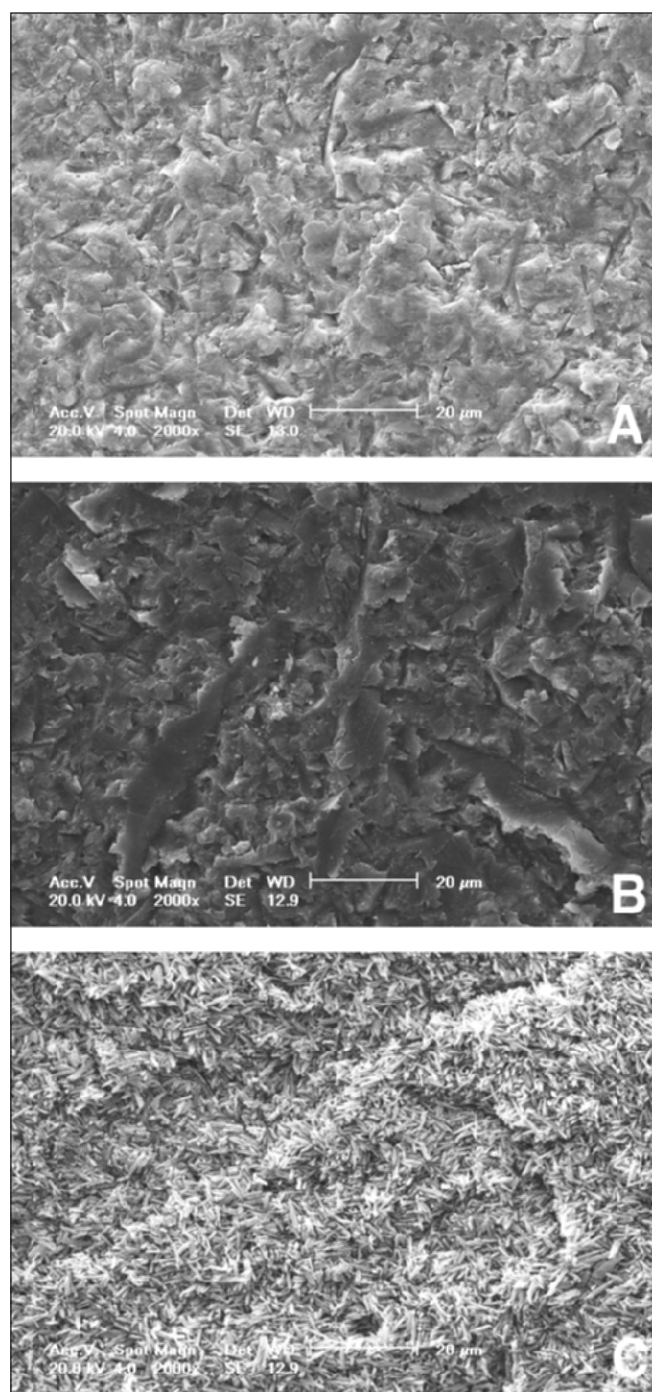
Figure 3. SEM of IPS Empress (a) Control (original magnification 2000x), (b) Airborne particle abrasion with 50- \mu\text{m} aluminum oxide for 15 seconds (original magnification 2000x), (c) Etching with 9.5% hydrofluoric acid for 20 seconds (original magnification 2000x).
