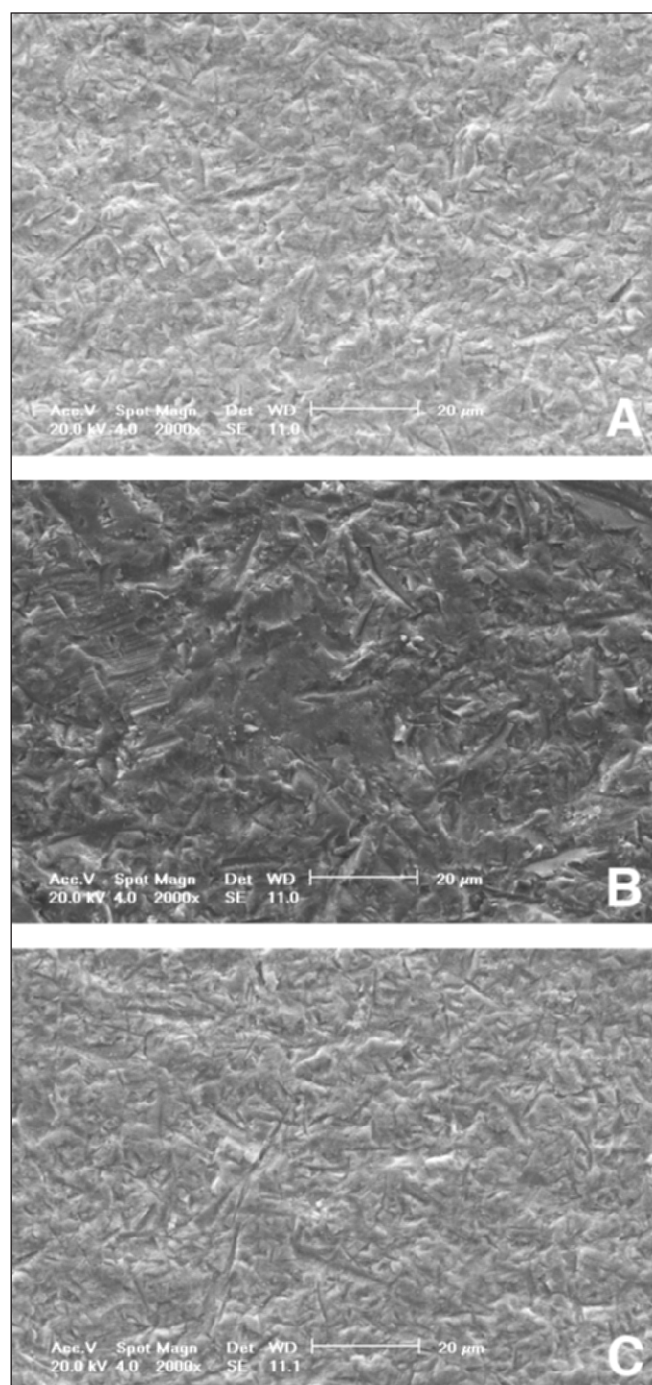
Figure 5. SEM of In-Ceram Alumina (a) Control (original magnification 2000x), (b) Airborne particle abrasion with 50- \mu m aluminum oxide for 15 seconds (original magnification 2000x), (c) Etching with 9.5% hydrofluoric acid for two minutes (original magnification 2000x).
