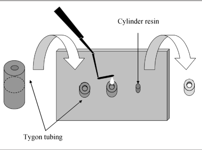
Figure 1. Scheme of the bonding procedure.
