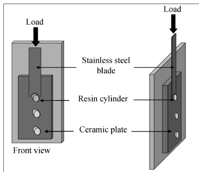
Figure 2. Schematic views of the micro-shear bond test.
