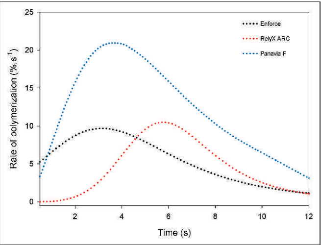
Figure 1. Representative polymerization rate profiles for the immediate light-activation mode.
