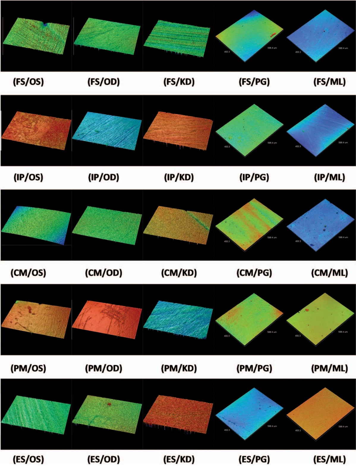
Figure 1. 3-D surface scans of representative samples of the different groups (10.3×; image size: 598.4 μm × 455.3 μm)
