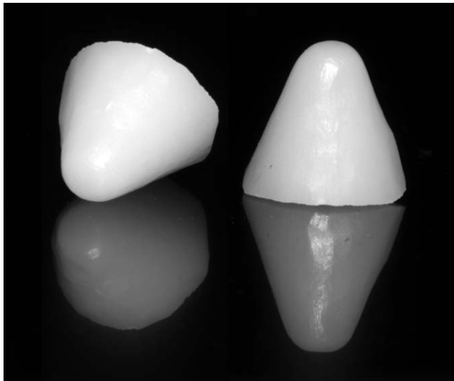
Figure 1. Standard zirconia cusps used as abraders in the chewing simulation test.
