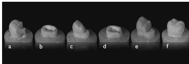
Figure 8. All specimens were analyzed and classified in one of the three failure modes: (a,b): Catastrophic, that is, tooth/root fracture that would require tooth extraction. (c,d): Possibly reparable, that is, cohesive/adhesive failure with fragment and minor damage, chip, or crack of the underlying tooth structure. (e,f): Reparable fracture, that is, cohesive or cohesive/adhesive fracture of restoration only.
