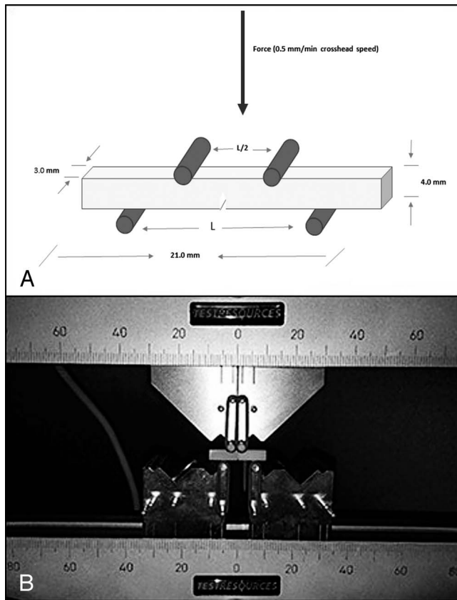
Figure 1. (A) Schematic illustration of fracture toughness specimen. L is the distance between the rollers in the four-point bending fixture. (B) Specimen placed on four-point bending fixture.
