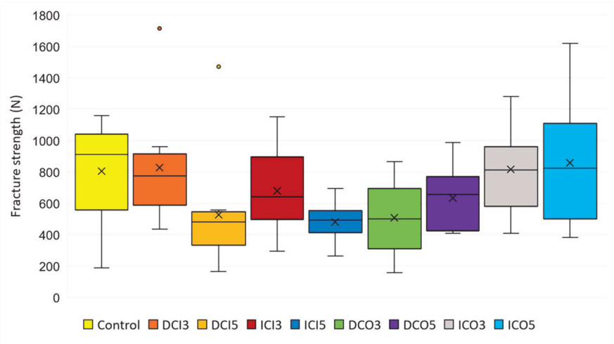
Figure 4. Fracture strength of the groups. Abbreviations: x = mean; ° = outlier.
